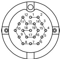
HOLE NUMBER ASSIGNMENTS FRONT VIEW
