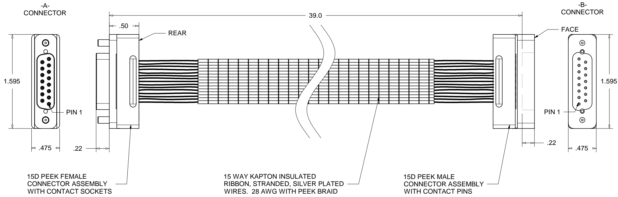
FACE VIEW
